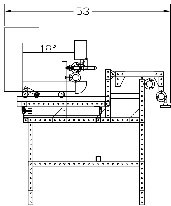
18" MACHINE W/ 8' TABLE
