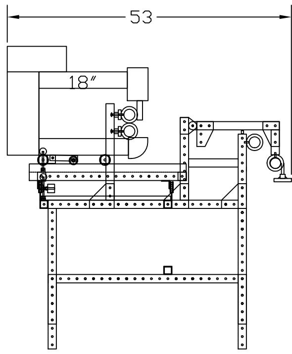
18" MACHINE W/ 12' TABLE
