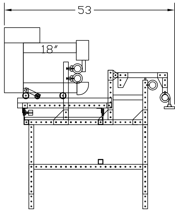
18" MACHINE W/ 10' TABLE
