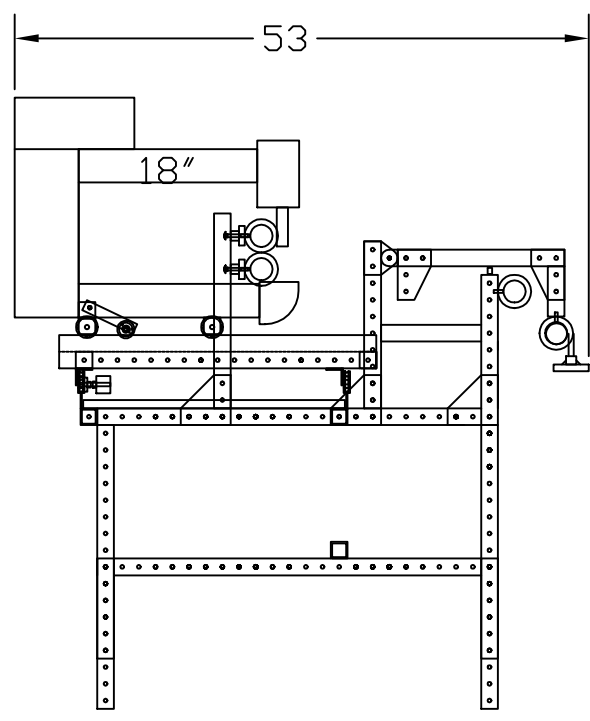
18" MACHINE W/ 14' TABLE
