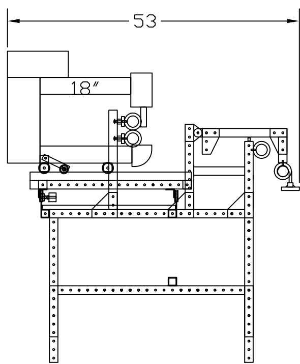
18" MACHINE W/ 6' TABLE
